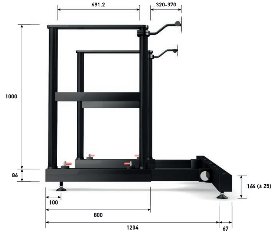
Side Elevation
